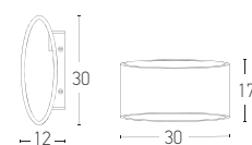
180020 D: 30 H:17 L:12 1xE27 MAX 40W Material: Concrete
