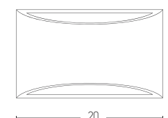
180025 D: 20 H:12 L:8.5 1xG9 MAX 25W Material: Gypsum Available Color: Pure White
