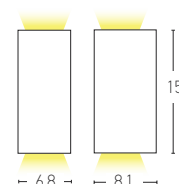
E 124 D: 6.8 H:15 L:8.1 2xGU10 MAX 35W Material: Aluminium-Glass Diffuser Available Color: Graphite IP 54
