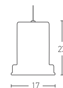
1580 D: Ø17 H:23 1x E27 MAX 40W Material: Concrete Available Color: Concrete Base: Chrome Available Cable: 120cm
