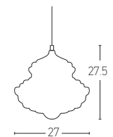
1675 D: Ø27 H:27.5 1xE27 MAX 40W Material: Opal Glass Available Color: White Available Cable: 130cm
