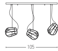
1541 D: Ø20x105 H:100 Base:105x6,5 3xG9 MAX 25W Material: Metal-Opal Glass Available Color: Black Matt Available Cable: 80cm
