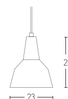
180086 D: Ø23 H:28 1x E27 MAX 40W Material: Aluminium-Wood Available Color: White Matt Available Cable: 150cm
