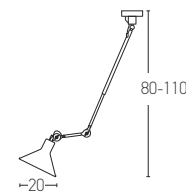
19219 D: H:80-110 Shade:Ø20 1xE27 MAX 40W Material: Metal-Aluminium Available Color: Black Matt-White
