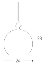
180098 D: Ø24 H:28 1x E27 MAX 40W Material: Aluminium Available Color: White Matt-Copper Available Cable: 150cm
