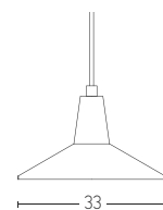
180085 D: Ø33 H:23 1x E27 MAX 40W Material: Aluminium-Wood Available Color: Black Matt Available Cable: 150cm
