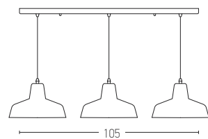
1653 D: 25x105 Base: 105 x6.5 3xE27 MAX 40W Material: Concrete Available Color: Concrete, Base: Black Matt Available Cable: 100cm
