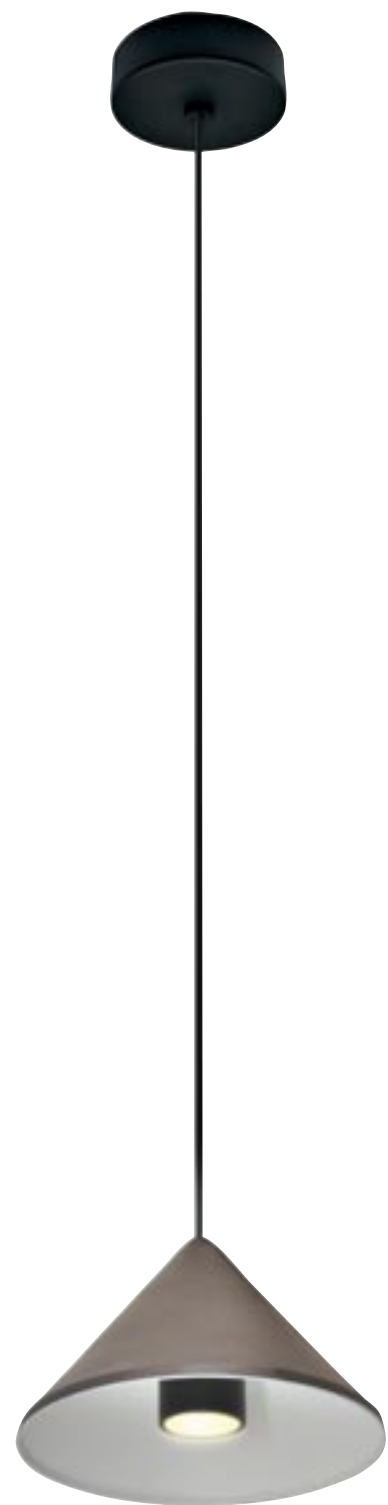
1911 D: Ø12 H:7.5 Stick: 2.7x6 Base: Ø8x3 6W LED, 3000K, 110Lumen/W Beam Angle: 18° Material: Metal-Aluminium Available Color: Black Matt-White Available Cable: 200cm
