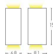
E 122 D: 6.8 H:15 L:8.1 2xGU10 MAX 35W Material: Aluminium-Glass Diffuser Available Color: Graphite IP 54
