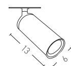
S056 D: Ø6x13 H:17 Recessed Base: Ø6 ☐ 1xGU10 MAX 35W Material: Aluminium Available Color: White Matt Special Feature: Recessed
