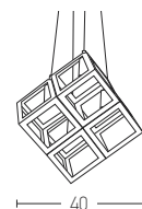
1678 D: 40x40 Base: Ø12 4x E27 MAX 40W Material: Metal Available Color: Black Matt Available Cable: 150cm
