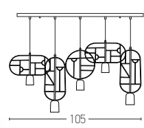
17028 D: 24x105 H:100 Base:105x6.5 5xGU10 MAX 25W Material: Metal Available Color: Black Matt Available Cable: 70cm
