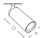
S057 D: Ø6x13 H:17 Recessed Base: Ø6 ☐ 1xGU10 MAX 35W Material: Aluminium Available Color: Black Matt Special Feature: Recessed
