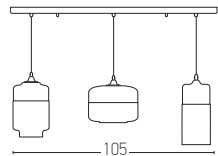
1519 D: 24x105 H:120 Base:105x6.5 3x E27 MAX 40W Material: Glass Available Color: Champagne-Black Matt Available Cable: 100cm
