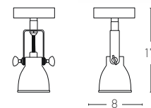
17141 D: Ø8 H:17 1xGU10, MAX 35W Material: Metal Available Color: Brown
