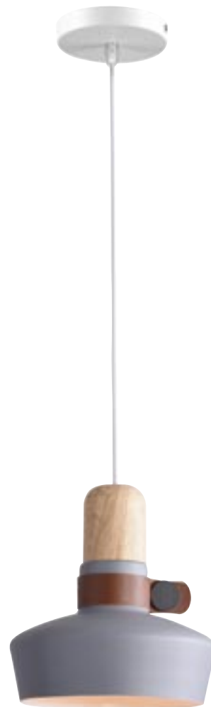
1991 D: Ø20 H:22 Base:Ø10 1xE27 MAX 40W Material: Metal-Leather-Wood Available Color: Grey Matt Available Cable: 200cm
