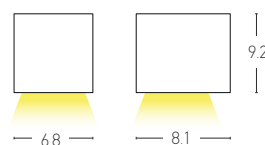
E 121 D: 6.8 H:9.2 L:8.1 1xGU10 MAX 35W Material: Aluminium-Glass Diffuser Available Color: Graphite IP 54
