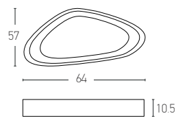
17019 D: Ø64x57 H:10.5 44W LED, 3000K, 80Lumen/W Material: Metal-Acrylic Available Color: White Matt
