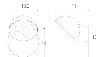
180044 D: Ø13.2 H:12 L:11 5W LED, 3000K, 80Lumen/W Material: Metal-Aluminium-Acrylic Available Color: Sandy White
