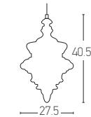
1674 D: Ø27.5 H:40.5 1xE27 MAX 40W Material: Opal Glass Available Color: White Available Cable: 130cm
