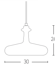
180097 D: Ø30 H:24 1x E27 MAX 40W Material: Aluminium Available Color: White Matt-Copper Available Cable: 150cm
