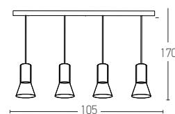
19123 D: 12.5x105 Base: 105x6.5 4xGU10 LED MAX 9W Material: Metal-Aluminium-Glass Available Color: Light Blue-Black Matt Available Cable: 150cm
