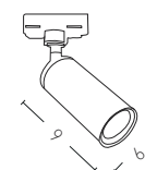
S067 D: Ø6 H:9 1xGU10 MAX 35W Material: Metal Available Color: Copper Rusty Special Feature: 3 Phase Adaptor
