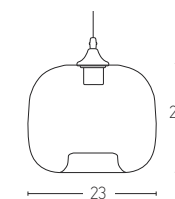
1574 D: Ø23 H:20 1xE27 MAX 40W Material: Glass Available Color: Brown-Green Available Cable: 150cm
