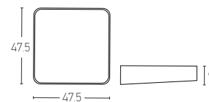
17017 D: 47.5x47.5 H:9 = 48W LED, 3000K, 90Lumen/W Material: Metal-Acrylic Available Color: Black Matt
