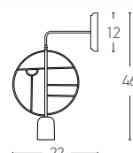
17030 D: 24 H:46 L:22 1xGU10 MAX 25W Material: Metal Available Color: Black Matt
