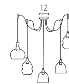
1501 D: Base: Ø12 5x E27 MAX 40W Material: Metal Available Color: Black Matt Available Cable: 150cm
