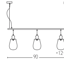
16109 D: 12x90 H:35 Glass: Ø12 3x E27 MAX 40W Material: Metal-Glass Available Color: Black Matt Available Cable: 100cm
