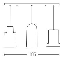
1584 D: 17x105 Base:105x6.5 3x E27 MAX 40W Material: Concrete Available Color: Concrete Base: Black Matt Available Cable: 100cm
