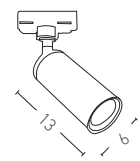
S059 D: Ø6 H:13 ☐ 1xGU10 MAX 35W Material: Aluminium Available Color: Black Matt Special Feature: 3 Phase Adaptor
