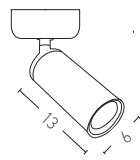
S054 D: Ø6x13 H:20 Base: Ø6 ☐ 1xGU10 MAX 35W Material: Aluminium Available Color: White Matt
