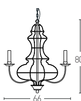
17115 D: Ø66 H:80 6xE14 MAX 40W Material: Metal Available Color: Rusty Brown Available Chain: 50 cm
