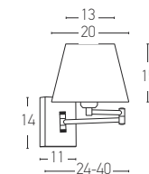
H-25W D: Base:11x14 L:24-40 Shade:20x13x15 1x E27 MAX 40W Material: Metal-Fabric Shade Available Color: Bronze-Beige Shade
