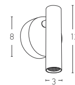
H-47 D: Stick:12x3 Base:Ø8 3W LED, 3000K, 80Lumen/W Material: Aluminium-Metal Available Color: Copper Switch: On/Off
