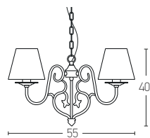
17123 D: Ø55 H:40 ⦿ 3x E14 MAX 40W Material: Metal-Fabric Shade Available Color: Brown-Gold Available Chain: 50 cm
