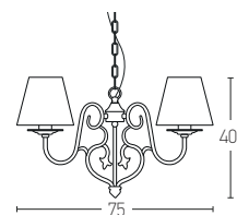
17125 D: Ø75 H:40 ⦿ 6x E14 MAX 40W Material: Metal-Fabric Shade Available Color: Brown-Gold Available Chain: 50 cm
