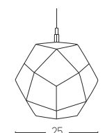
1684 D: Ø25 H:25 1x E27 MAX 40W Material: Metal-Stainless Steel Available Color: Copper Base: Black Matt Available Cable: 150cm
