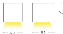
E 123 D: 6.8 H:9.2 L:8.1 1xGU10 MAX 35W. Material: Aluminium-Glass Diffuser Available Color: Graphite IP 54
