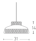
18113 D: Ø31x14 1xE27 MAX 40W Material: Concrete Available Color: Concrete Base: Chrome Available Cable: 120cm
