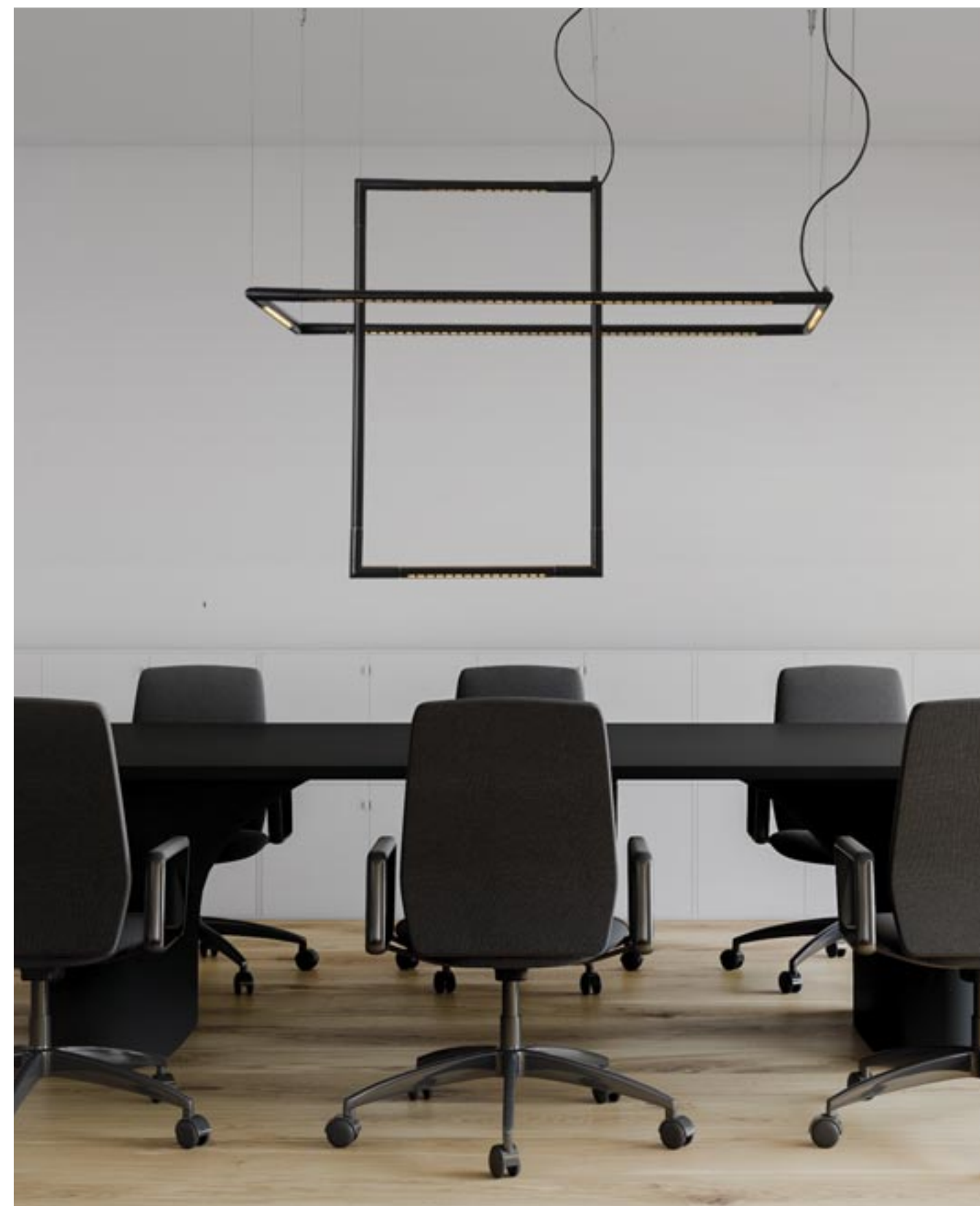
19236 ㄱ D: 111x51, 81x51, Base: 50x7x5 Tube: Ø2.4 ≡ 30W LED, 3000K, 90Lumen/W Special Feature: Movable Tube Material: Metal-Aluminium-Diffuser Available Color: Sandy Black Available Cable: 200cm
