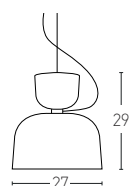
17033 D: Ø27 H:29 Base:Ø12 1x E27 MAX 40W Material: Aluminium Available Color: Dark Blue-Maroon Available Cable: 100cm
