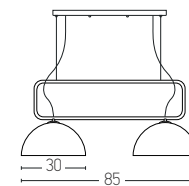
17092 D: 85x30 Shade: Ø30 2x E27 MAX 40W Material: Metal-Aluminium Available Color: Black Matt-Golden Leaf Available Cable: 70 cm
