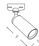
S064 D: Ø6 H:9 1xGU10 MAX 35W Material: Brass Available Color: Real Brass Special Feature: 3 Phase Adaptor
