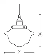
16118 D: Ø21 H:25 1xE27 MAX 40W Material: Glass-Metal Available Color: Bronze-Black Matt Available Cable: 150cm
