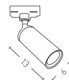
S062 D: Ø6 H:13 1xGU10 MAX 35W Material: Aluminium Available Color: Black Matt Special Feature: 3 Phase Adaptor
