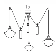
16116 ㄣ D: Base: Ø15 3xE27 MAX 40W Material: Glass-Metal Available Color: Bronze-Black Matt Available Cable: 150cm
