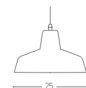
1655 D: Ø25 H:16 1xE27 MAX 40W Material: Concrete Available Color: Concrete Base: Chrome Available Cable: 100cm
