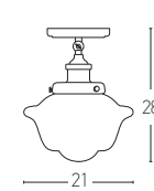
16117 D: Ø21 H:28 1xE27 MAX 40W Material: Glass-Metal Available Color: Bronze-Black Matt
