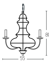
17116 D: Ø55 H:80 3xE14 MAX 40W Material: Metal Available Color: Rusty Brown Available Chain: 50 cm
