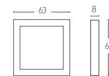
18148-B ㄣ D: 63x63x8 72W LED, 3000K, 140Lumen/W Material: Aluminium-Acrylic Available Color: Sandy Black
