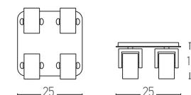
16188 D: 25x25 H:17 4xGU10 MAX 40W Material: Metal Available Color: Black Matt-Chrome
