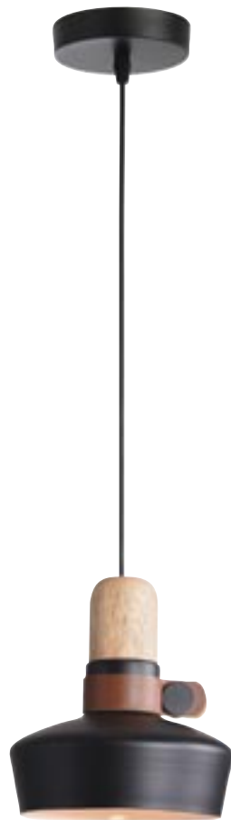
1990 D: Ø20 H:22 Base:Ø10 1xE27 MAX 40W Material: Metal-Leather-Wood Available Color: Black Matt Available Cable: 200cm
