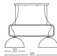
17155 D: 85x30 Shade: Ø30 2x E27 MAX 40W Material: Metal-Aluminium Available Color: Black Matt Available Cable: 70 cm
