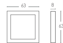
18148-W ㄣ D: 63x63x8 72W LED, 3000K, 140Lumen/W Material: Aluminium-Acrylic Available Color: Sandy White
