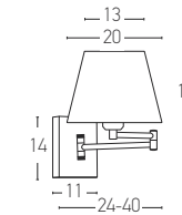
H-24W D: Base:Ø11x14 L:24-40 Shade:20x13x15 1x E27 MAX 40W Material: Metal-Fabric Shade Available Color: Chrome Matt-Beige Shade
