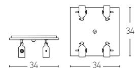
1480 ㄱ D: Ø34x34 L:11 4xE27 MAX 40W Material: Brass-Wood
