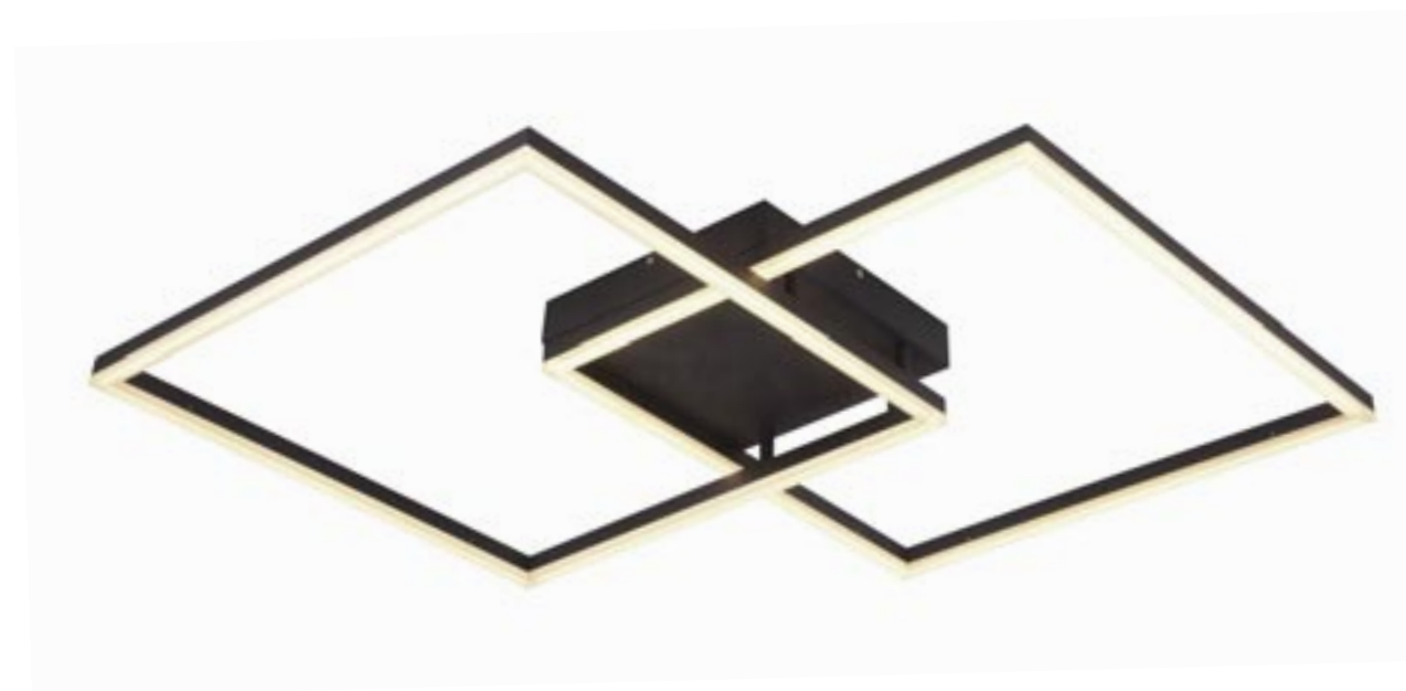
17006 D: 65x99 H:9 60W LED, 3000K, 80Lumen/W Special Feature: Dimmable / Phase cut Leading or Trailing Edge Material: Metal-Aluminium-Acrylic Available Color: Black Matt
