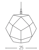
1683 D: Ø25 H:25 1x E27 MAX 40W Material: Metal-Stainless Steel Available Color: Gold Base: Black Matt Available Cable: 150cm
