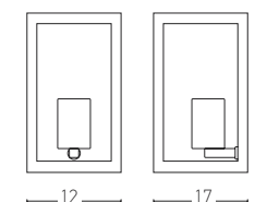
1699 D: 12 H:20 L:17 1x E27 MAX 40W Material: Metal-Glass Available Color: Black Matt
