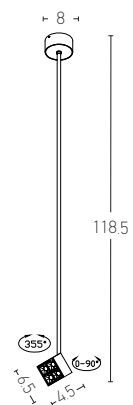
1929 D: 6.5x6.5x4.5 H:118.5, Base: Ø8x4 7W LED, 3000K, 110Lumen/W Special Feature: Standard Legnth Material: Metal-Aluminium Available Color: Sandy Black
