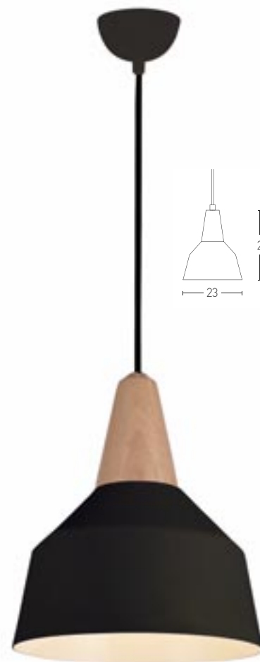
180088 D: Ø23 H:28 1x E27 MAX 40W Material: Aluminium-Wood Available Color: Black Matt Available Cable: 150cm
