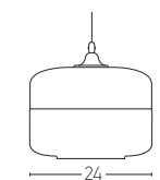
1516 D: Ø24 H:23 1x E27 MAX 40W Material: Glass Available Color: Champagne-Black Matt Available Cable: 150cm
