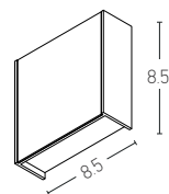
1922 D: 8.5 H:8.5 L:2.7 ≡ 3W LED, 3000K, 110Lumen/W Material: Aluminium-Diffuser Available Color: Sandy White-Black
