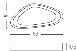
17018 D: Ø50x46 H:10.5 30W LED, 3000K, 80Lumen/W Material: Metal-Acrylic Available Color: White Matt
