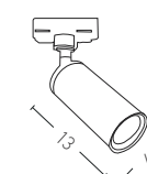
S062-15 | S062-24 | S063-40 D: Ø6 H:13 9W LED, 3000K 80Lumen/W, CRI:90 Special Feature: Included LED driver Beam Angle: 15/24/40° Material: Aluminium Available Color: Black Matt Special Feature: 3 Phase Adaptor
