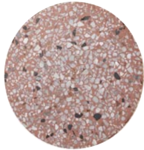
1943 D: Ø20 L:6 ≡ 10W LED, 3000K, 70Lumen/W Material: Mosaic Available Color: Pink
