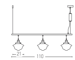
16115 ㄣ D: 21x110 H:35 3xE27 MAX 40W Material: Glass-Metal Available Color: Bronze-Black Matt Available Cable: 100cm
