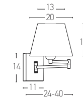
H-24B D: Base:Ø11x14 L:24-40 Shade:20x13x15 1x E27 MAX 40W Material: Metal-Fabric Shade Available Color: Chrome Matt-Black Shade
