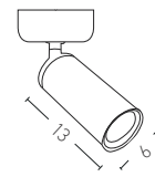
S055 D: Ø6x13 H:20 Base: Ø6 ☐ 1xGU10 MAX 35W Material: Aluminium Available Color: Black Matt
