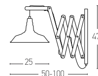
16166 D: Ø25 H:47 L:50-100 1xE27 MAX 40W Material: Metal-Wood Available Color: Black
