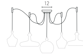
180099 D: Base: Ø12 5x E27 MAX 40W Material: Aluminium Available Color: White Matt-Copper Available Cable: 150cm
