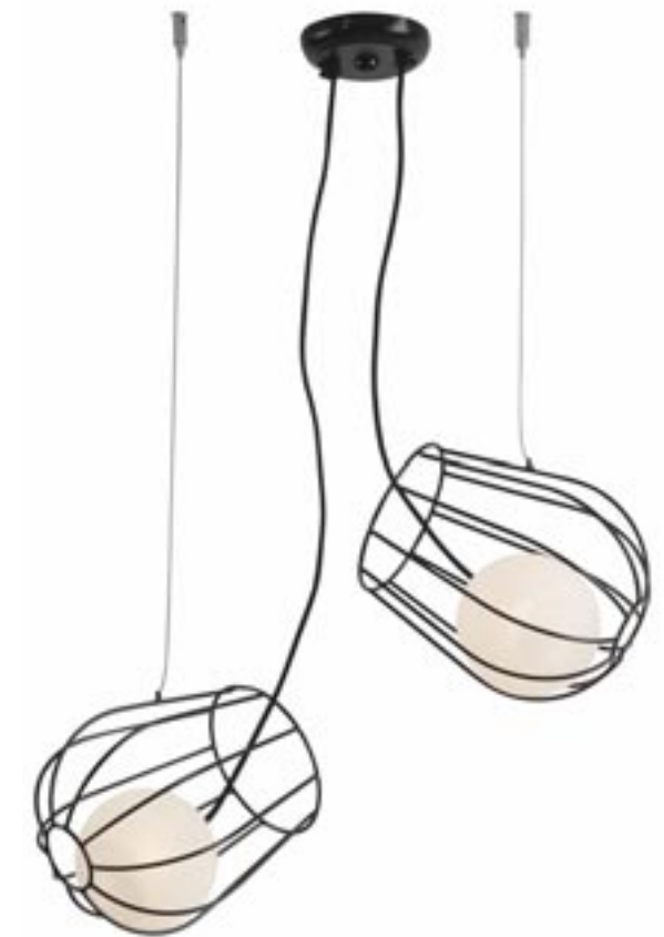
1542 D: Base: Ø12 2xG9 MAX 25W Material: Metal-Opal Glass Available Color: Black Matt Available Cable: 100cm
