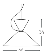
17032 D: Ø46 H:34 Base:Ø12 1x E27 MAX 40W Material: Aluminium Available Color: Grey-Light Blue Available Cable: 100cm
