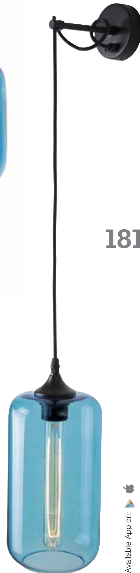
1648 D: Ø13.5 H:120 L:20 Base: Ø8 1xE27 MAX 40W Material: Glass Available Color: Light Blue Available Cable: 150cm
