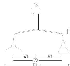
180084 D: 120x11, Base: 16x5.5 2x E27 MAX 40W Material: Metal-Aluminium-Wood Available Color: Black Matt Available Cable: 80cm
