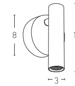
H-48B D: Stick:12x3 Base:Ø8 3W LED, 3000K, 80Lumen/W Material: Aluminium-Metal Available Color: Black Matt Switch: On/Off
