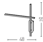
1945 D: 48 H: 55 L:10 Base:15.5x5.5 20W LED, 3000K, 100 Lumen/W Material: Metal-Aluminium-Acrylic Available Color: Black Matt
