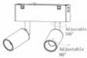
18203 ≡ 2x5W LED 48V, 3000K, 80Lumen/W Beam Angle: 36° Spot Size: 3,5x6,1cm Available Color: Sandy Black
